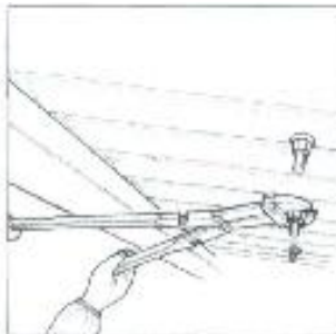
Cut the bolts while avoiding contact with the asbestos cement. Double-wrap large pieces in 1000-gauge polythene sheeting and seal with duct tape
