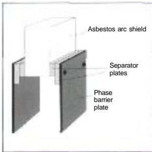
Arc shield
